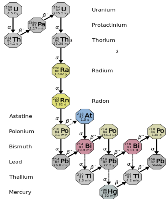
Figure 1. ^{238}\text{U} Decay Series. Note daughter products ^{226}\text{Ra} , ^{222}\text{Rn} , and ^{210}\text{Pb} .
